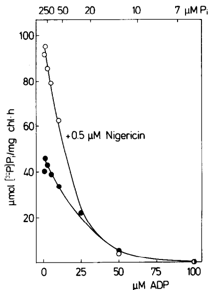
Fig.2. The initial rate of dark ATP hydrolysis at constant initial ATP concentration ( 50 \mu\text{M} ) and constant initial phosphate potential ( 60 \text{ kJ/mol} ) adjusted by the addition of ADP and \text{P}_i at varying concentrations with constant c_{\text{ADP}}c_{\text{P}_i} = 6.25 \times 10^{-10} \text{ M}^2 . [\gamma\text{-}^{32}\text{P}]\text{ATP} , ADP and \text{P}_i \pm 0.5 \mu\text{M} nigericin were added together after 2 min preillumination ( 250 \text{ W} \cdot \text{m}^{-2} ) following 15 s dark treatment.
